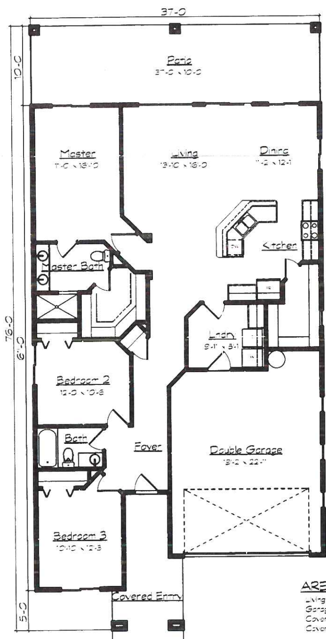
Floor Plan A. 2 Car
